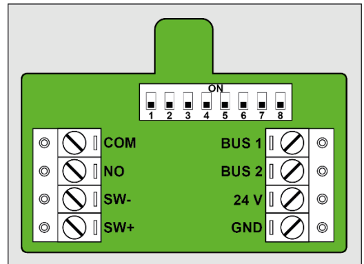
Abb. 17: Anschlüsse Video-Innenstation
